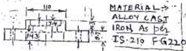
SLEEVE & BEARING HOUSING EXPANSION TYPE
