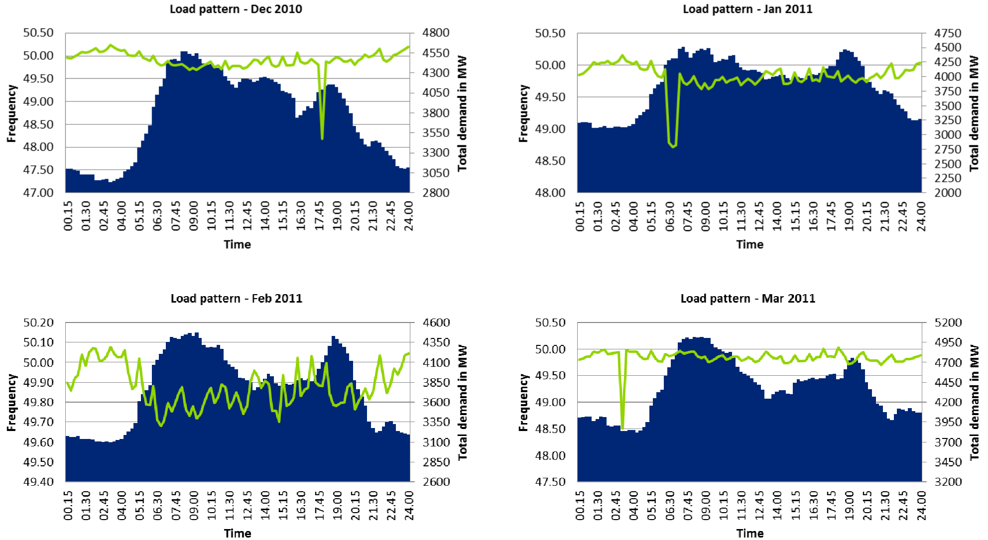
Figure 3: Loading pattern and frequency variation of PSPCL for December to March period
