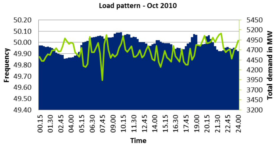
Figure 2: Loading pattern and frequency variation of PSPCL for August to November period
