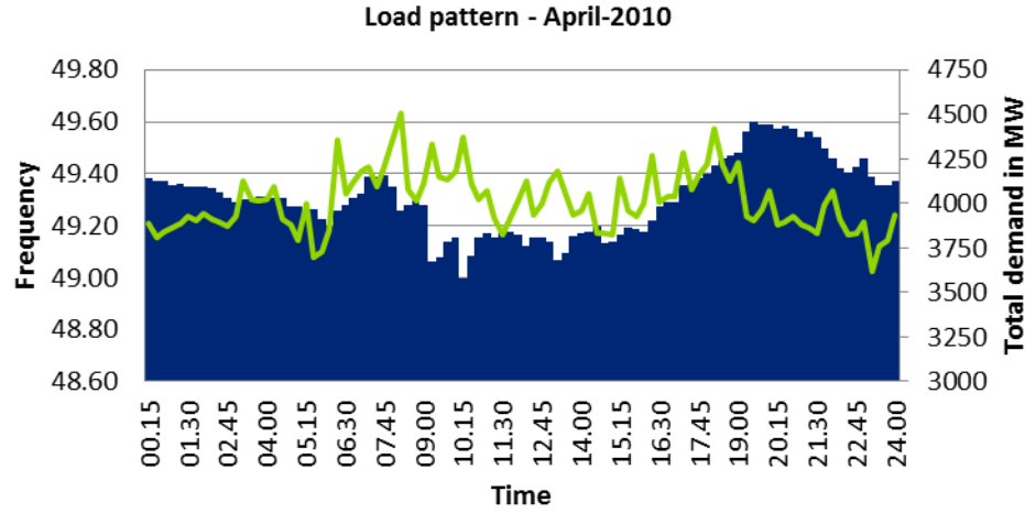
Figure 1: Loading pattern and frequency variation of PSPCL for April to July period
