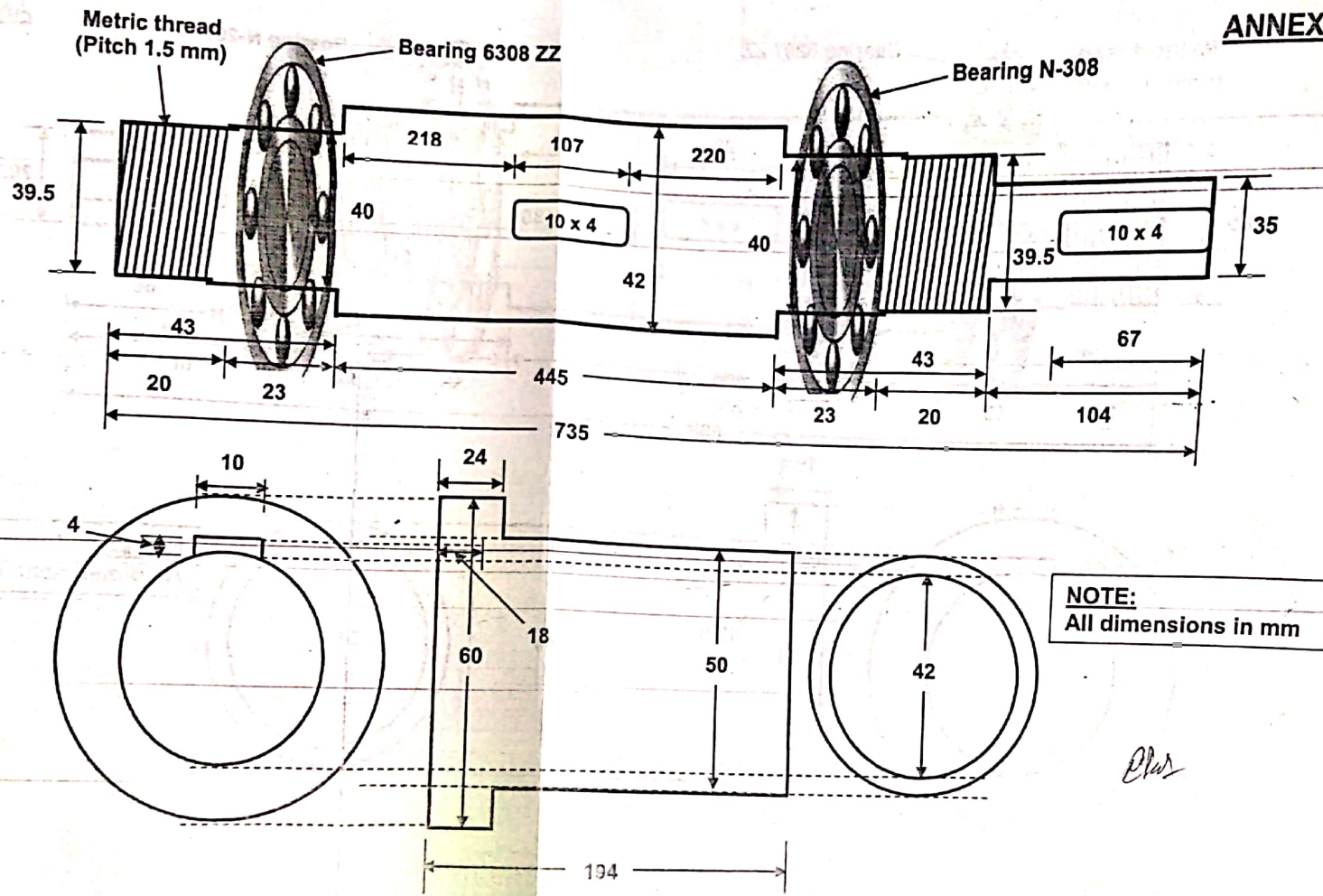
ROUGH SKETCH OF SHAFT & SHAFT SLEEVE OF BEST & CRAMPTON MAKE PUMP MODEL: SDC 100/125, CAPACITY 30 M 3 /HR., HEAD 40 MWG, RPM-1470, HORIZONTAL, SINGLE-STAGE
