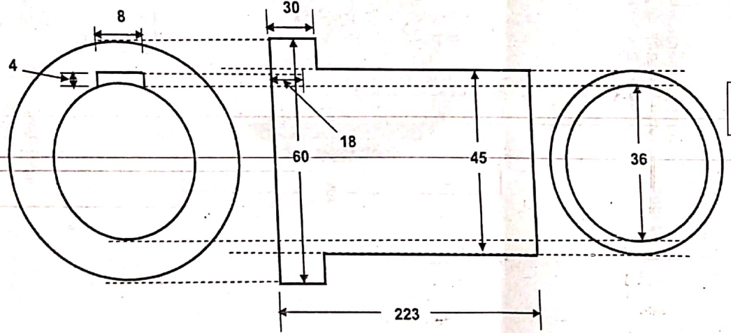
ROUGH SKETCH OF SHAFT & SHAFT SLEEVE OF BEST & CROMPTON MAKE PUMP MODEL: SDB-150/200, CAPACITY 300 M 3 /HR, HEAD 30 MWC, RPM-1470, HORIZONTAL, SINGLE-STAGE
