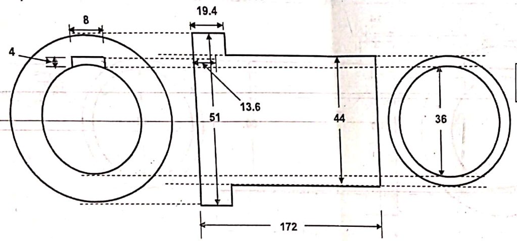
ROUGH SKETCH OF SHAFT & SHAFT SLEEVE OF BEST & CROMPTON MAKE PUMP MODEL: BWC 80/100 - 300, CAPACITY 100 M 3 /HR., HEAD 30 MWC, RPM-1470, HORIZONTAL, SINGLE-STAGE
