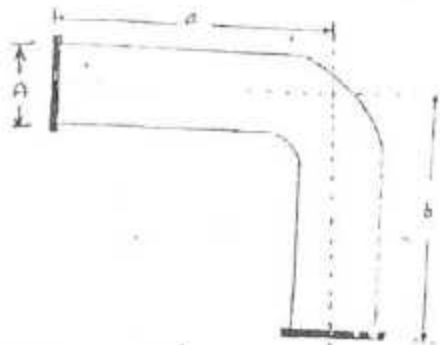
MSRL 90° BEND
