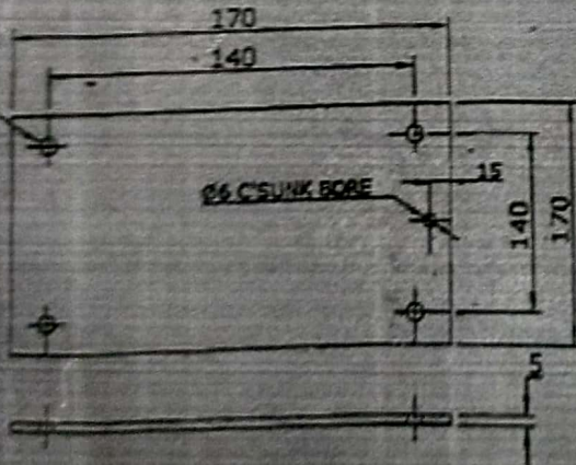
MOUNTING PLATE DETAIL
